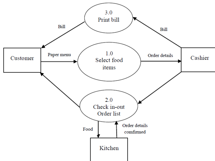
Figure 15: Diagram 0 of Existing System.
