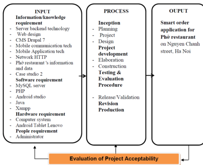
Figure 12: Input-Process-Out (IPO) Chart.
