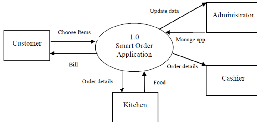
Figure 16: Context Diagram of Proposed System.
