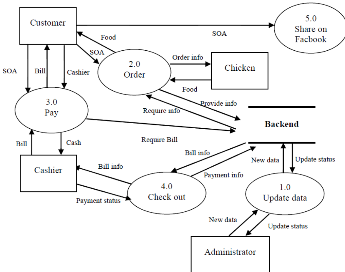
Figure 17: Diagram 0 of Proposed System.
